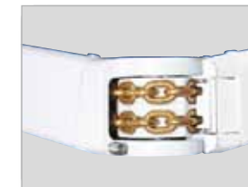
to protect them from corrosion the strong double steel-link chains are recessed into the elbow joints of the folding arms
